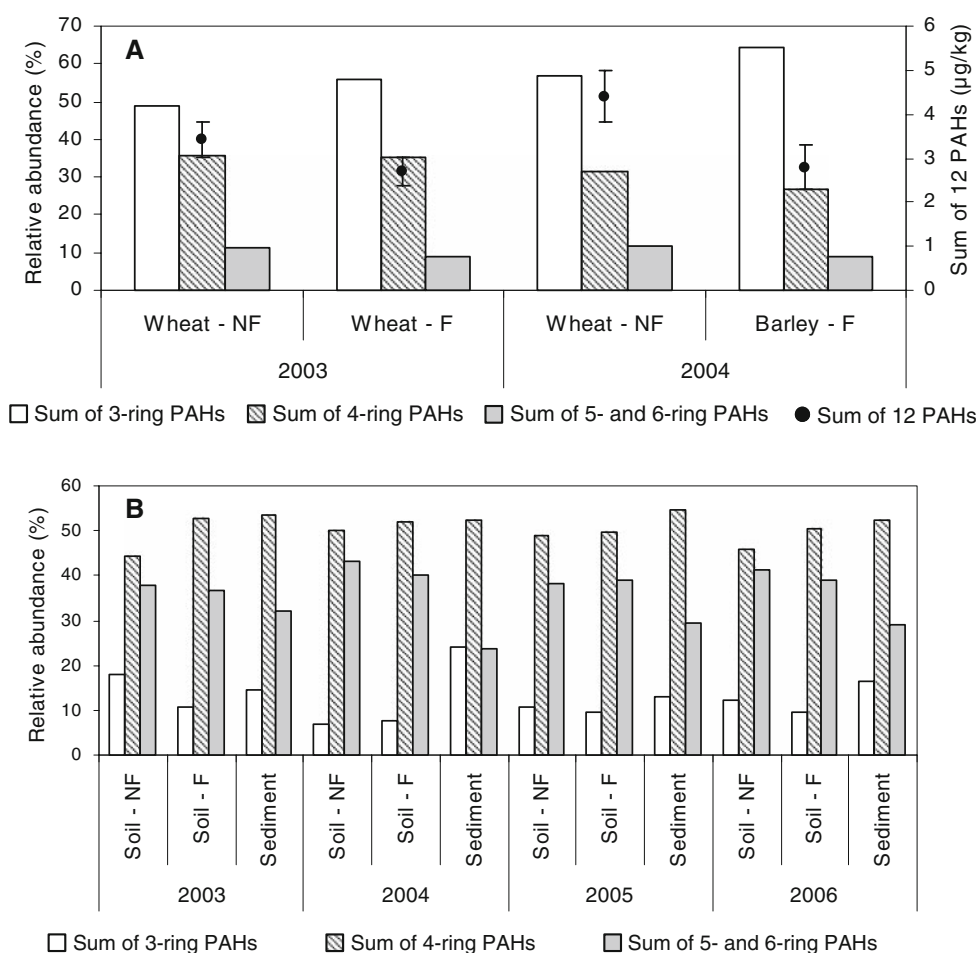
Fig. 2 (a) Relative abundance of PAH groups and PAHs content in cereals, (b) relative abundance of PAH groups in soil and sediment. NF = non-flooded area, F = flooded area, Sum of 3-ring PAHs = sum of Phe and Ant, Sum of 4-ring PAHs = sum of Flt, Pyr, B[a]A and Chr, Sum of 5- and 6-ring PAHs = sum of B[b]F, B[k]F, B[a]P, DB[ah]A, B[g,h,i]P and I[1,2,3-cd]P
